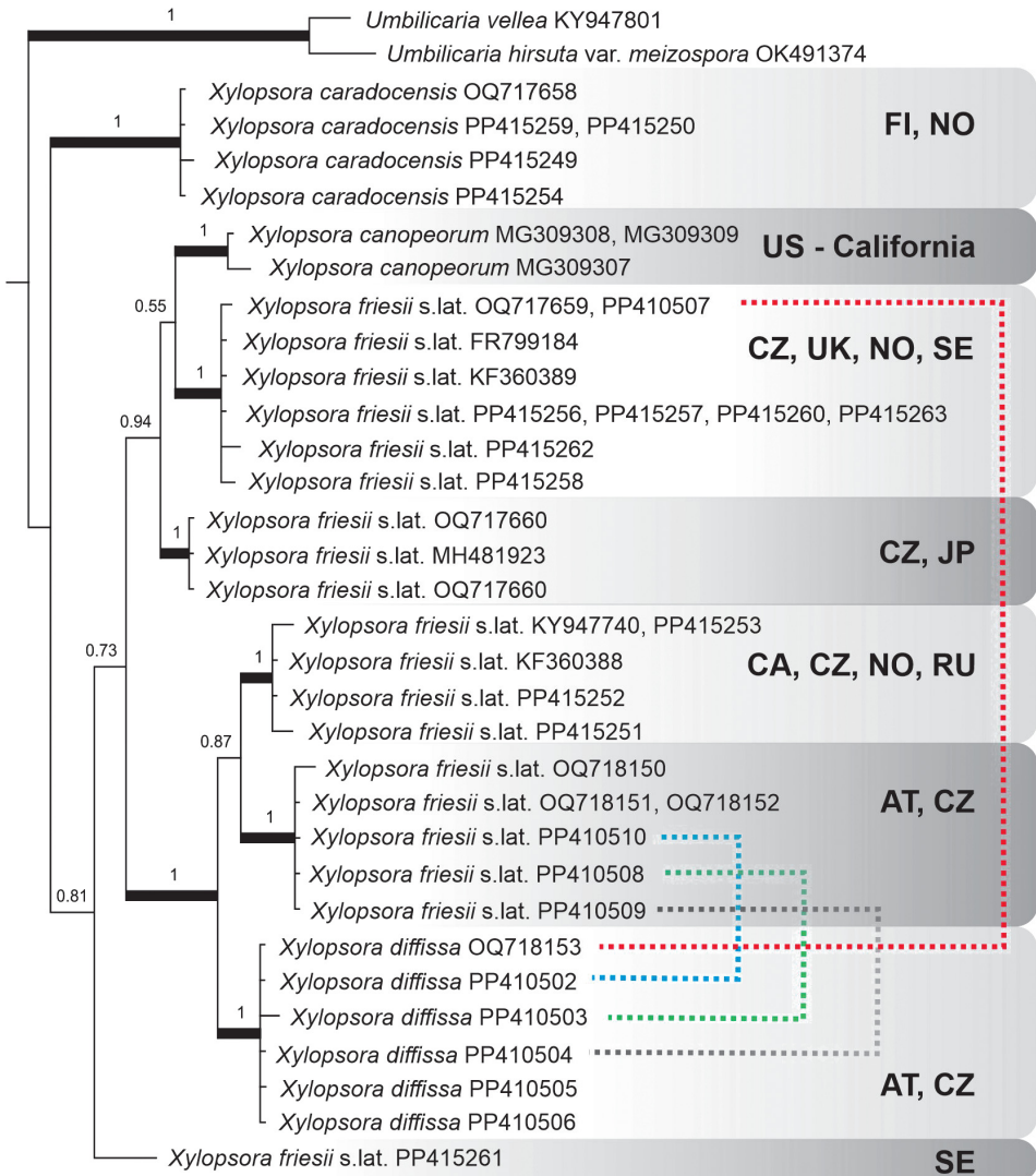
Fig. 16. Phylogenetic tree of Xylopsora based on ITS sequence data showing positions of Xylopsora diffissa and several lineages of X. friesii s. lat. GTR model with gamma distribution and proportion of invariable sites was used as a model of sequence evolution. The tree was constructed using Bayesian inference run for 144000 generations, and was rooted with Umbilicaria . Dotted lines connect the sequences of X. diffissa and X. friesii s. lat. occurring together in individual specimens and forming "mechanical hybrids". Country codes for sequenced specimens are given for each Xylopsora clade.
